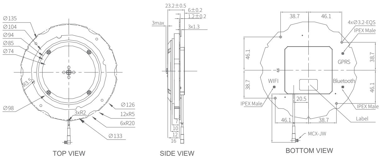
AT410 GNSS Antenna LCY4N01A Structure Drawing (mm)
