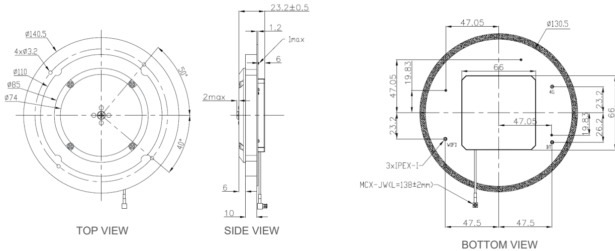
AT410 GNSS Antenna LC14N57A Structure Drawing (mm)
